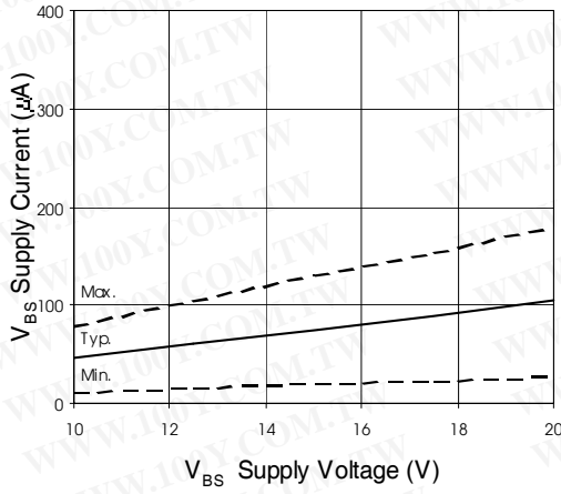
Figure 19B. VBS Supply Current vs. Supply Voltage
