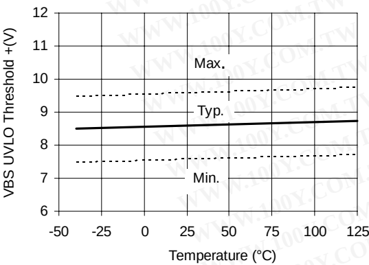
Figure 25 VBS Undervoltage Threshold (+) vsTemperature
