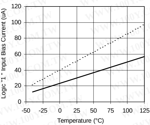
Figure 23A Logic “1” Input Current vs Temperature
