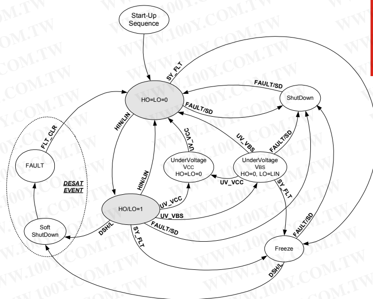
STATE DIAGRAM
