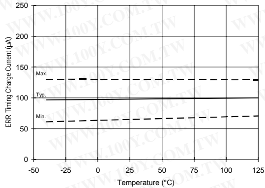
Figure 31A. ERR Timing Charge Current vs. Temperature
