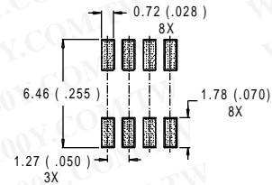
RECOMMENDED FOOTPRINT
