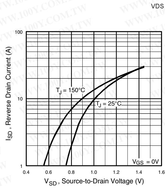
Fig 4. Typical Source-Drain Diode Forward Voltage
