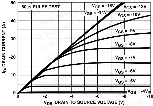
FIGURE 6. SATURATION CHARACTERISTICS
