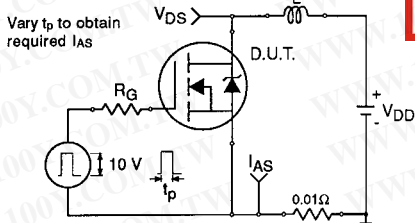
Fig 12a. Unclamped Inductive Test Circuit
