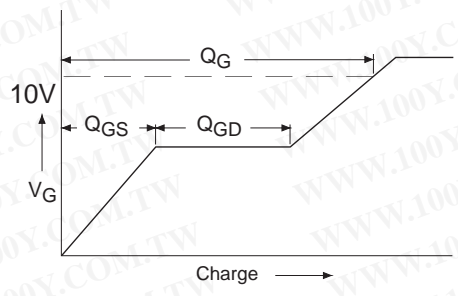
Fig 9a. Basic Gate Charge Waveform
