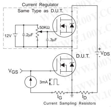
Fig 15a. Gate Charge Test Circuit
