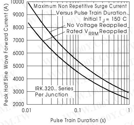
Fig. 31 - Maximum Non-Repetitive Surge Current
