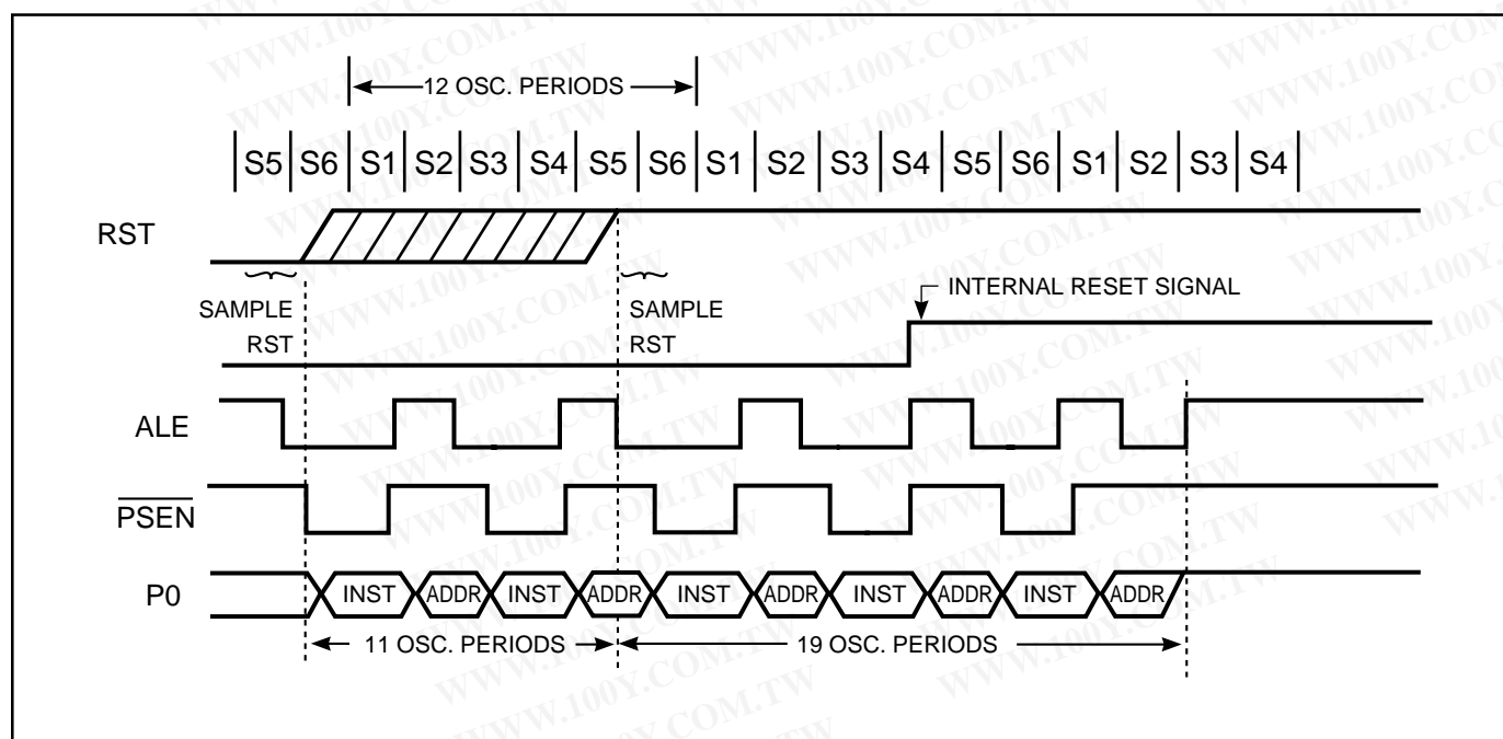
Figure 22. Reset Timing
