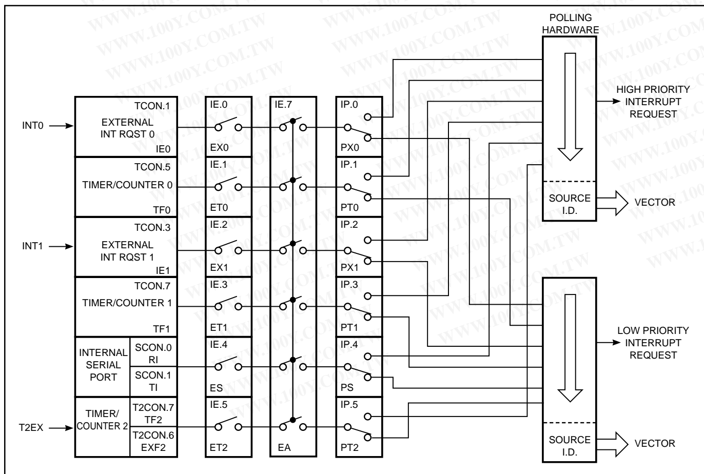
Figure 19. Interrupt System
