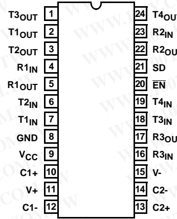
HIN236 (SOIC) TOP VIEW
