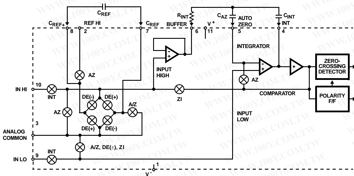
FIGURE 3. ANALOG SECTION OF ICL7135
