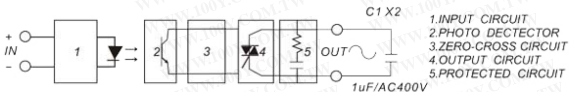
EQUIVALENT CIRCUIT
