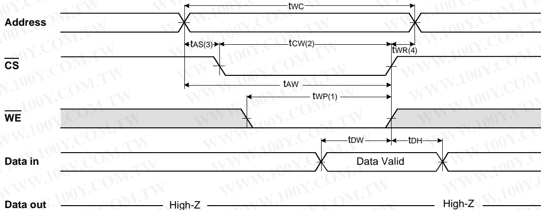
TIMING WAVEFORM OF WRITE CYCLE(2) (CS Controlled)
