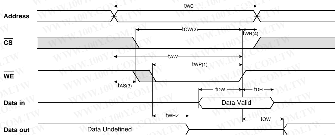
TIMING WAVEFORM OF WRITE CYCLE(2) (CS Controlled)
