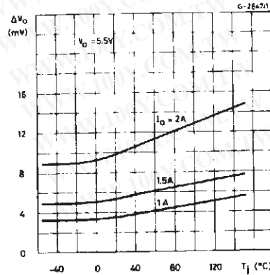
Figure 10. Voltage Load Regulation vs. Junction Temperature.
