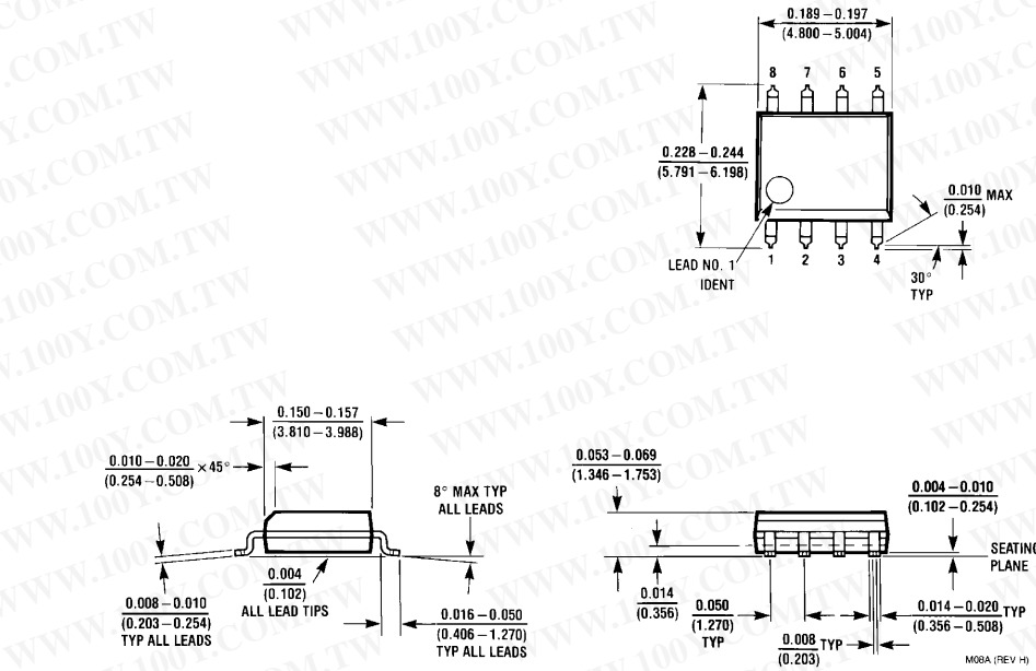
SO Package (M) Order Number LF351M NS Package Number M08A
