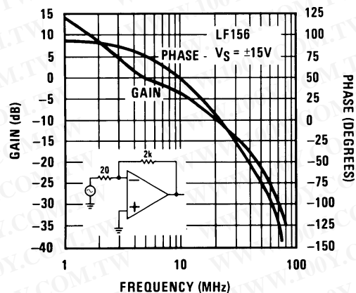
Bode Plot
