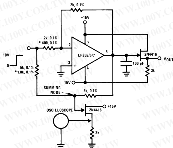
Settling Time Test Circuit
