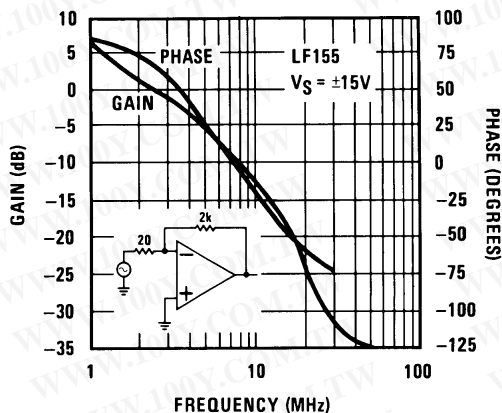
Bode Plot
