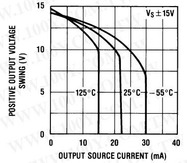
Positive Current Limit
