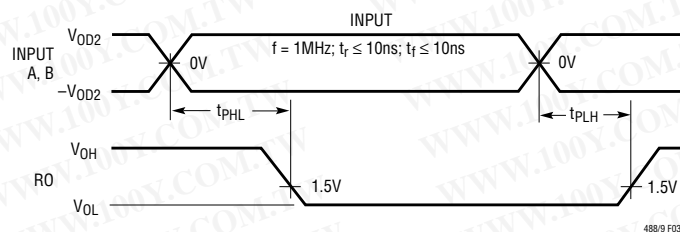
Figure 3. Receiver Propagation Delays
