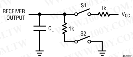
Figure 2. Receiver Enable and Disable Timing Test Circuit
