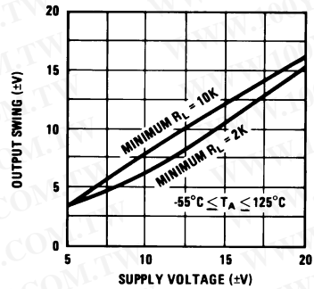
Output Swing
