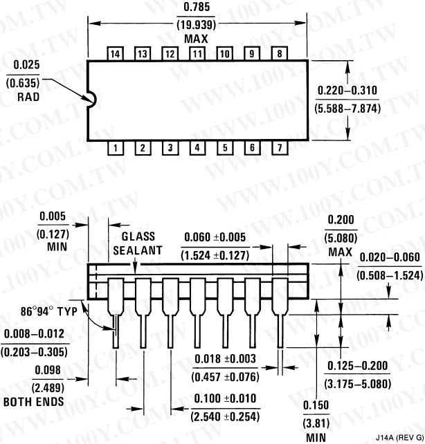
Ceramic Dual-In-Line Package (J) Order Number LM101AJ-14/883 NS Package Number J14A
