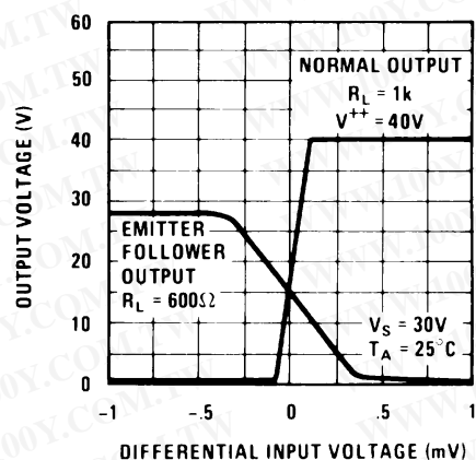
Transfer Function
