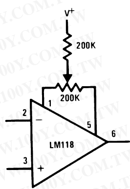
Offset Balancing
