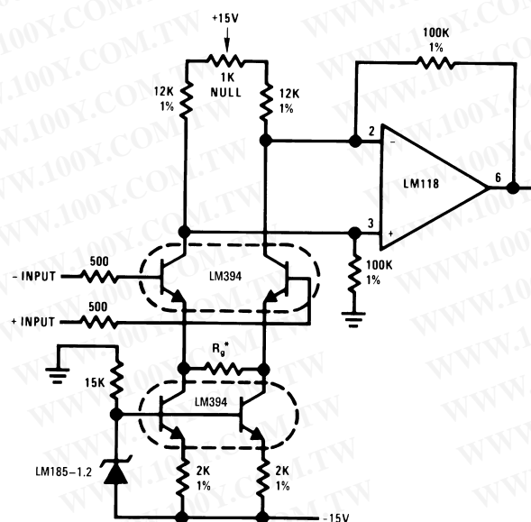
Instrumentation Amplifier
