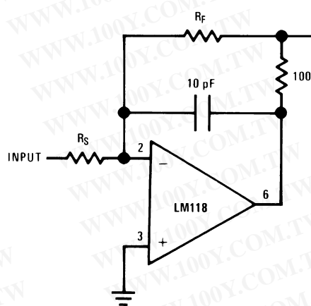
Isolating Large Capacitive Loads
