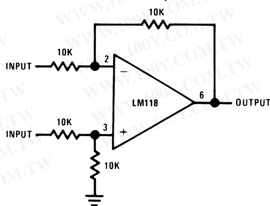
Differential Amplifier
