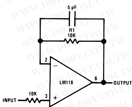
Fast Voltage Follower (Note 11)
