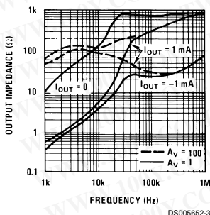
Output Impedance
