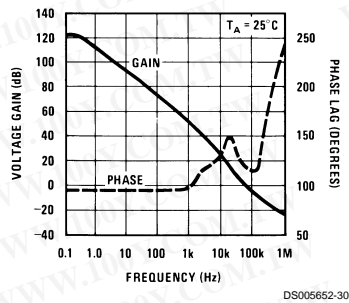
Frequency Response
