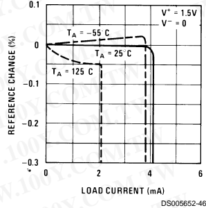
Output Saturation
