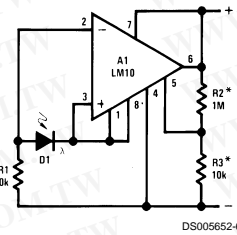
Light Level Sensor
