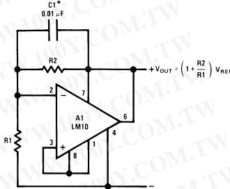
Shunt Regulator
