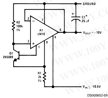
Negative Regulator
