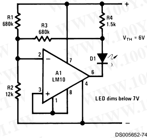
Battery-level Indicator
