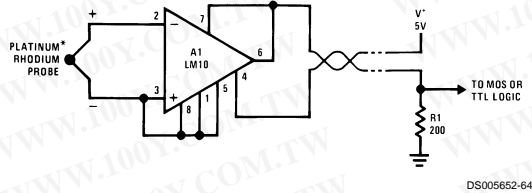
Flame Detector
