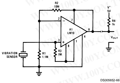
Remote Amplifier
