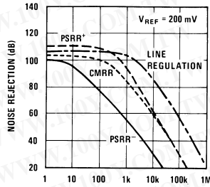
Noise Rejection
