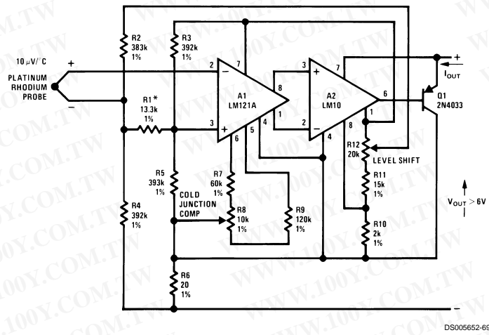
Precision Thermocouple Transmitter
