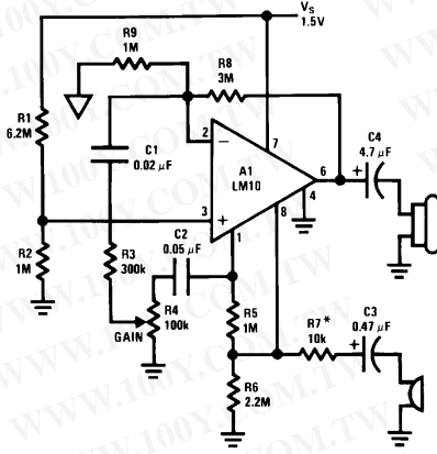
Microphone Amplifier
