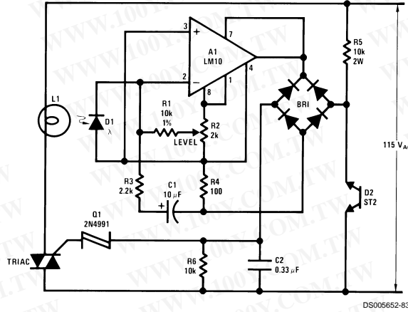
Light-level Controller
