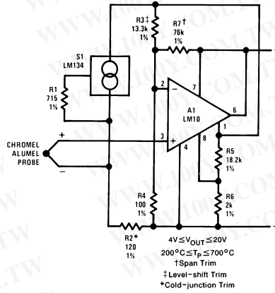
Remote Thermocouple Amplifier
