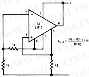
Current Regulator
