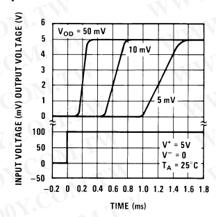
Comparator Response Time For Various Input Overdrives
