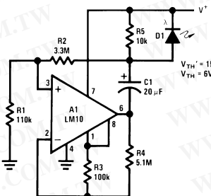
Double-ended Voltage Monitor
