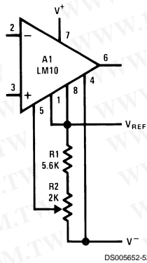
Limited Range
