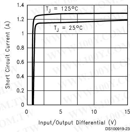
Short-Circuit Current
