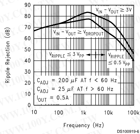
LM1117-ADJ Ripple Rejection
