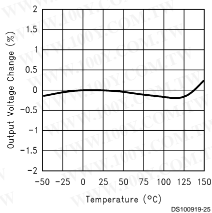
Temperature Stability
