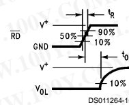
FIGURE 9. TRI-STATE Test Circuits and Waveforms
