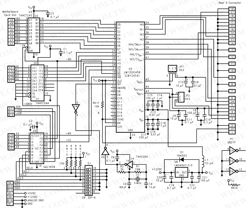
FIGURE 16. Schematic for the LM12(H)45/8 Evaluation Interface Board for XT and AT Style Computers, Order Number LM12458EVAL
