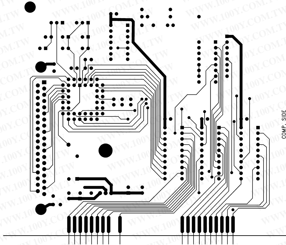
FIGURE 21. LM12(H)454/8 Evaluation/Interface Board Component-Side Layout Positive
