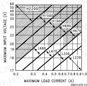
FIGURE 6. LM2575(HV)-15
