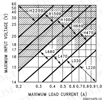
FIGURE 5. LM2575(HV)-12
