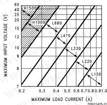
FIGURE 4. LM2575(HV)-5.0
