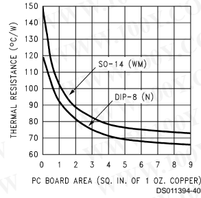
Junction to Ambient Thermal Resistance
