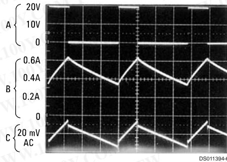
Continuous Mode Switching Waveforms
