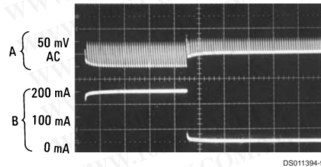
250 mA Load Transient Response for Discontinuous Mode Operation. L = 68 \mu H , C_{OUT} = 470 \mu F
