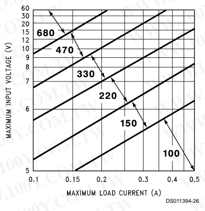
FIGURE 4. LM2574HV-3.3 Inductor Selection Guide
