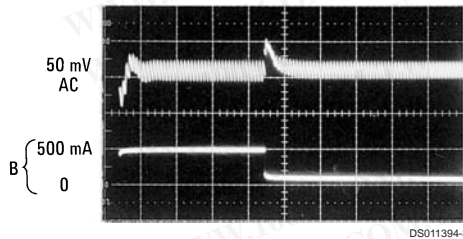
500 mA Load Transient Response for Continuous Mode Operation. L = 330 \mu H , C_{OUT} = 300 \mu F
