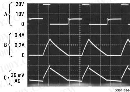
Discontinuous Mode Switching Waveforms
