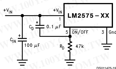
FIGURE 14. Delayed Startup
