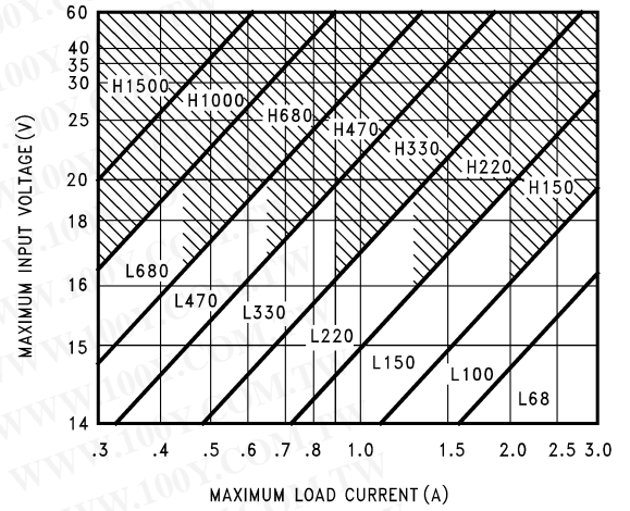
FIGURE 5. LM2576(HV)-12
