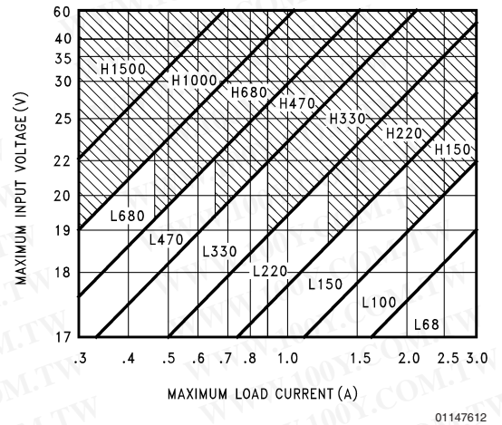
FIGURE 6. LM2576(HV)-15
