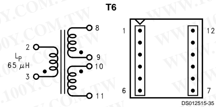
Top View FIGURE 20. Coilcraft Q4438-B (Surface Mount)
