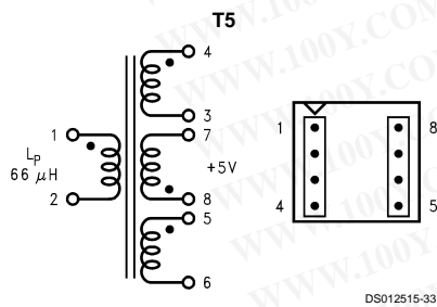
Top View FIGURE 18. Coilcraft Q4338-B
