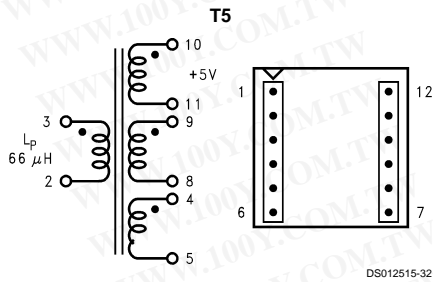
Top View FIGURE 17. Coilcraft Q4437-B (Surface Mount)
