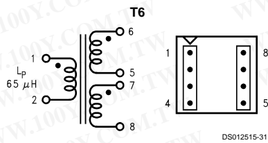
Top View FIGURE 16. Coilcraft Q4339-B
