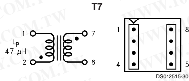
Top View FIGURE 15. Coilcraft S6000-A
