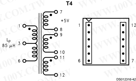
FIGURE 28. Renco RL-5535
