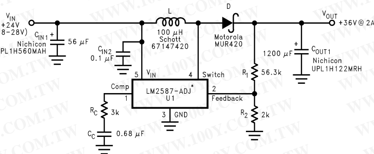
FIGURE 39. +24V to +36V Boost Regulator
