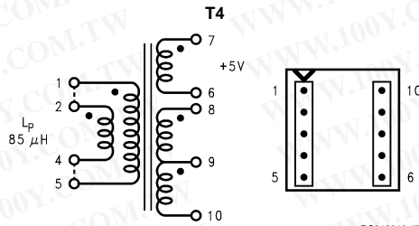
FIGURE 32. Schott 67140930
