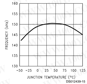
Switching Frequency
