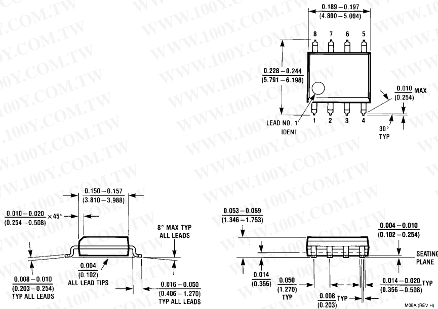
8-Lead (0.150" Wide) Molded Small Outline Package, JEDEC Order Number LM2671M-3.3, LM2671M-5.0, LM2671M-12 or LM2671M-ADJ NS Package Number M08A
