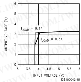
Dropout Voltage—3.3V Option
