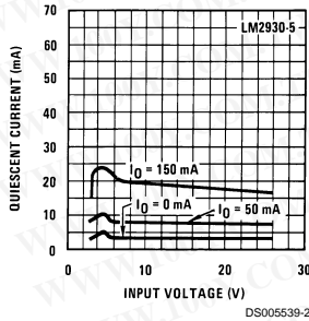
Quiescent Current
