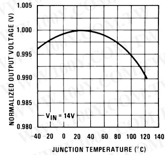
Output Voltage (Normalized to 1V at Tj=25°C)
