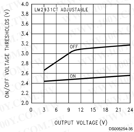
On/Off Threshold
