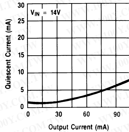
Quiescent Current
