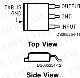
TO-263 Surface-Mount Package
