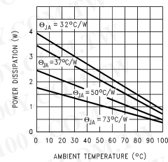
Maximum Power Dissipation (TO-263) (Note 3)
