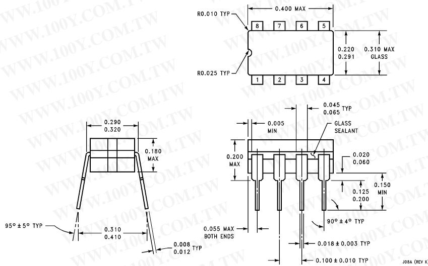
Cavity Dual-In-Line Package (J) Order Number LM111J-8, LM111J-8/883 or LM211J-8 NS Package Number J08A
