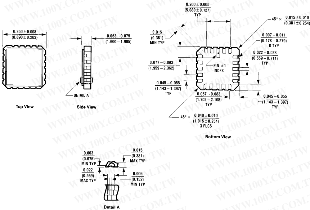
Order Number LM111E/883 NS Package Number E20A
