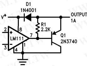
Comparator and Solenoid Driver
