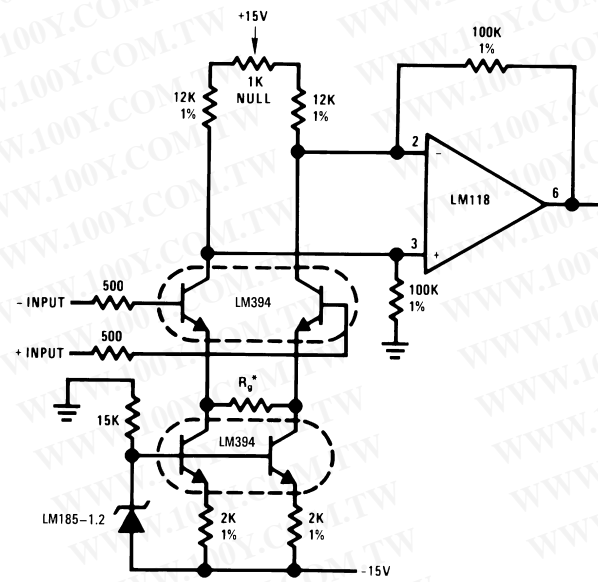
Instrumentation Amplifier
