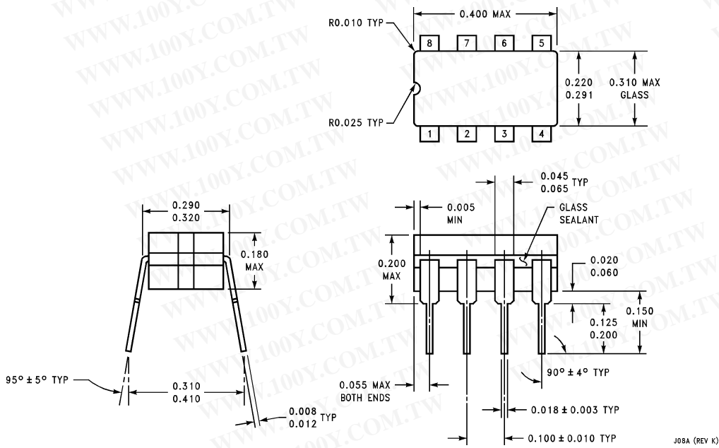
Ceramic Dual-In-Line Package (J) Order Number LM118J-8/883 NS Package Number J08A
