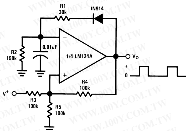
Pulse Generator
