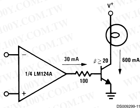
Lamp Driver
