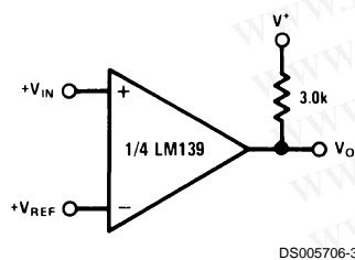
Basic Comparator
