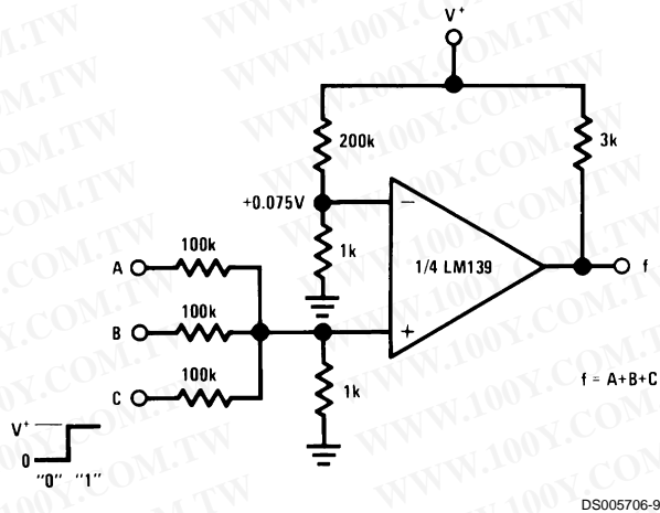
OR Gate
