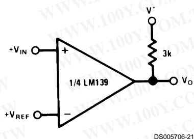
Basic Comparator
