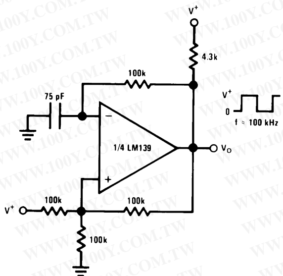
Squarewave Oscillator
