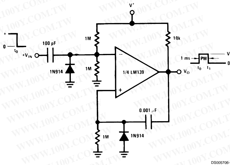
One-Shot Multivibrator
