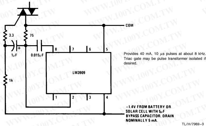
Triac Trigger
