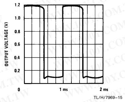
Note: Output voltage through a 10k load to ground.
