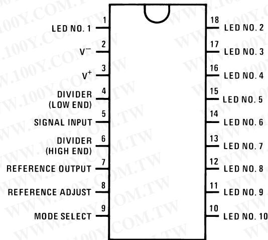
Dual-in-Line Package
