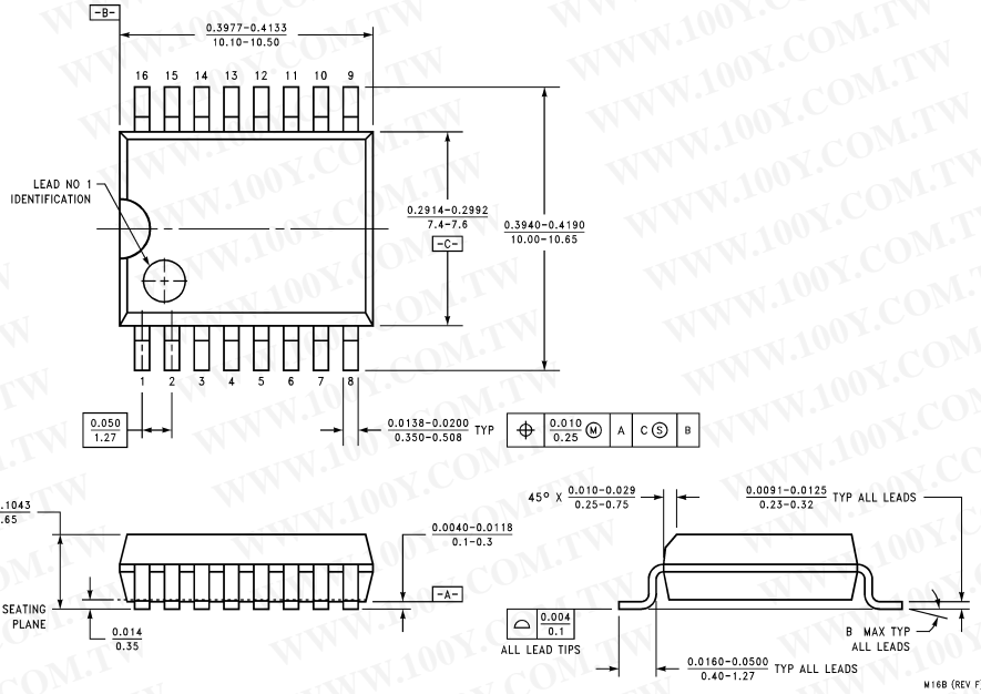
16-Lead (0.300" Wide) Molded Small Outline Package, JEDEC Order Number LM4863M NS Package Number M16B
