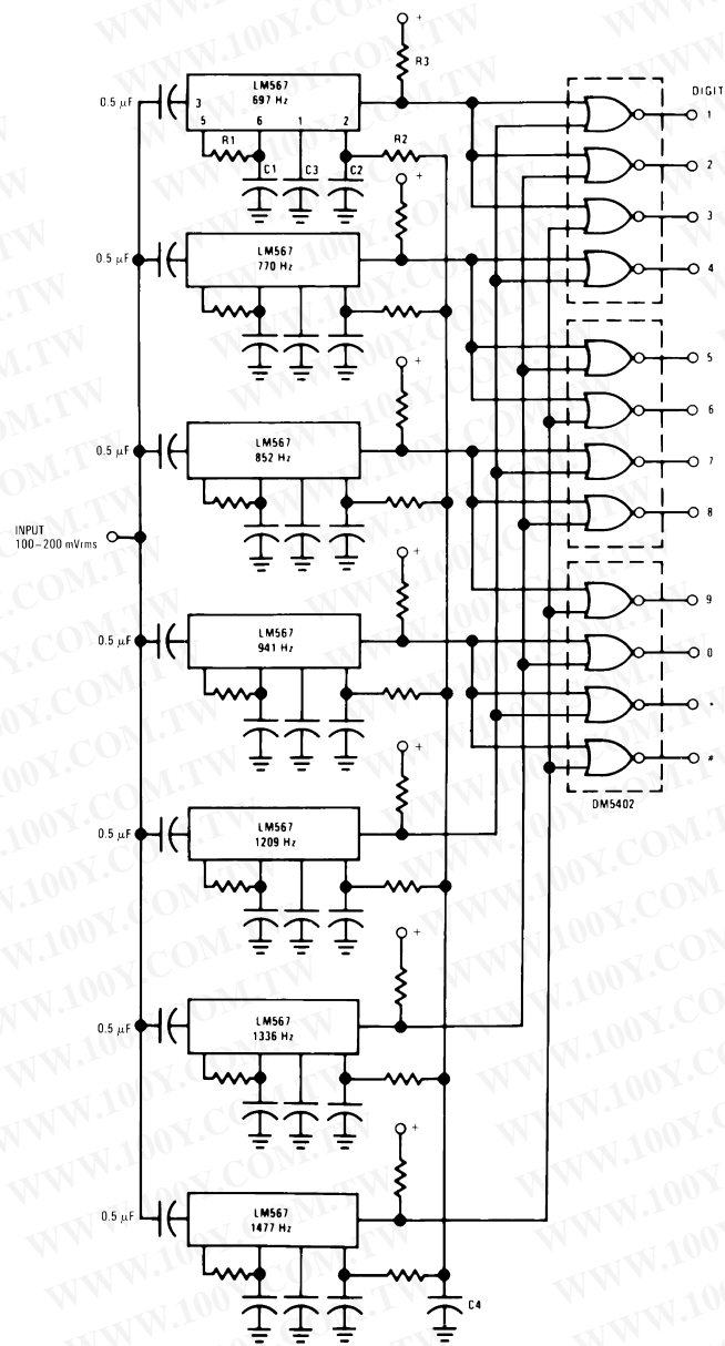
Touch-Tone Decoder
