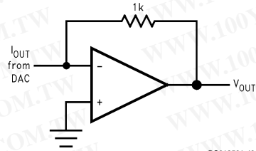
I-to-V Converters
