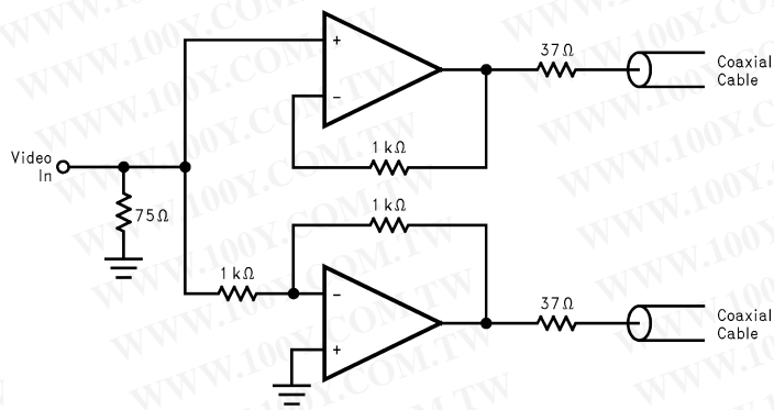
Differential Line Driver
