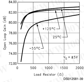
Large Signal Voltage Gain vs Load
