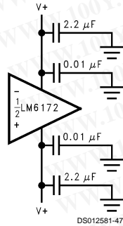
FIGURE 5. Power Supply Bypassing
