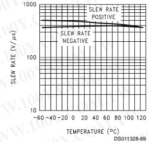
SLEW RATE vs TEMPERATURE A_V = -1 ; R_L = 150\Omega, V_S = \pm 5\text{V}
