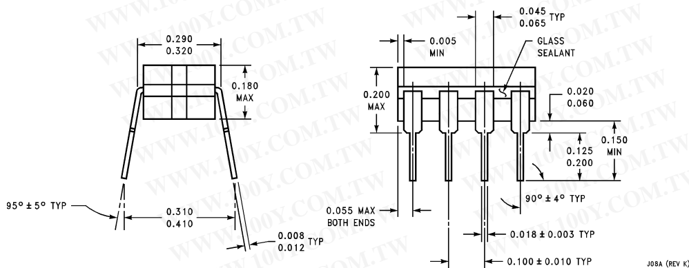
8-Pin Ceramic Dual-In-Line Package Order Number LM6181AM/J883 NS Package Number J08A
