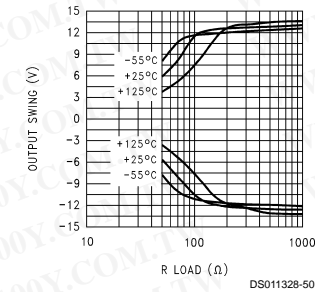
OUTPUT SWING vs R_{LOAD} PULSED, V_S = \pm 15\text{V}, I_{IN} = \pm 200\ \mu\text{A}, V_{IN+} = 0\text{V}
