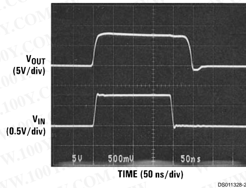
FIGURE 11. Closed-Loop Overdrive Recovery Time of 30 ns from Exceeding Output Voltage Range from Circuit in Figure 10
