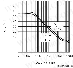
PSRR ( V_S^+ ) vs FREQUENCY
