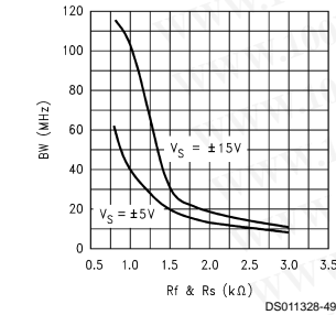
BANDWIDTH vs R_f & R_S A_V = -1, R_L = 1\text{ k}\Omega
