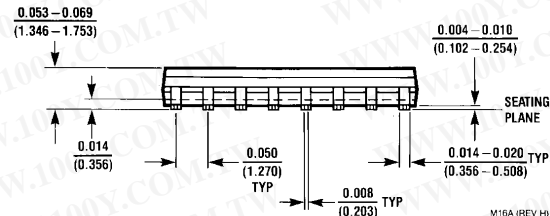
Small Outline Package (M) Order Number LM6181IM or LM6181AIM NS Package Number M16A
