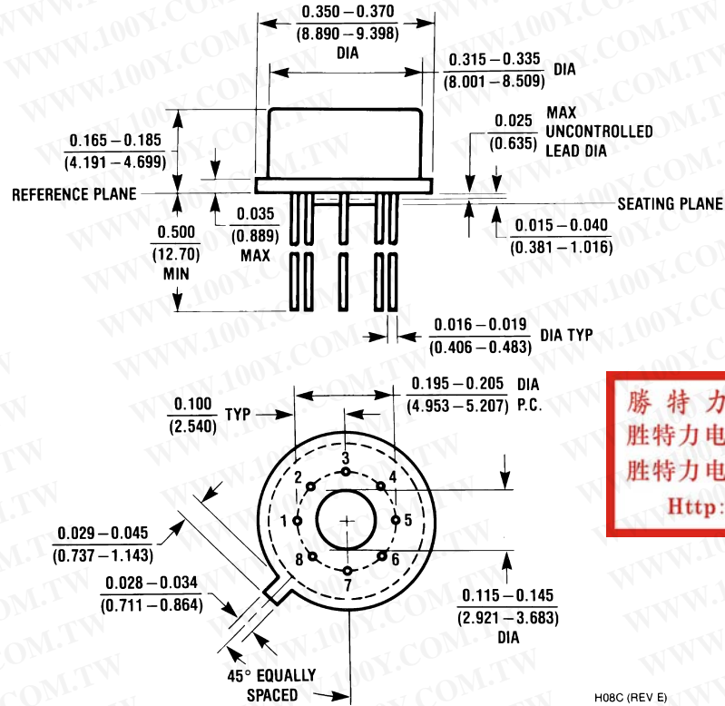
8-Pin Metal Can Package (H) Order Number LMC6001AIH or LMC6001BIH NS Package Number H08C
