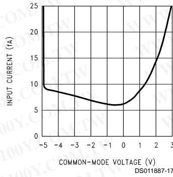
Input Current vs V_{CM} V_S = \pm 5V
