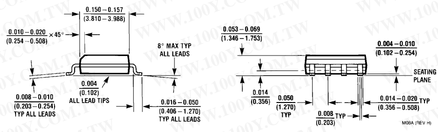
Small Outline Dual-In-Line Pkg. (M) Order Number LMC662AIM, LMC662CM, LMC662AIMX or LMC662CMX NS Package Number M08A
